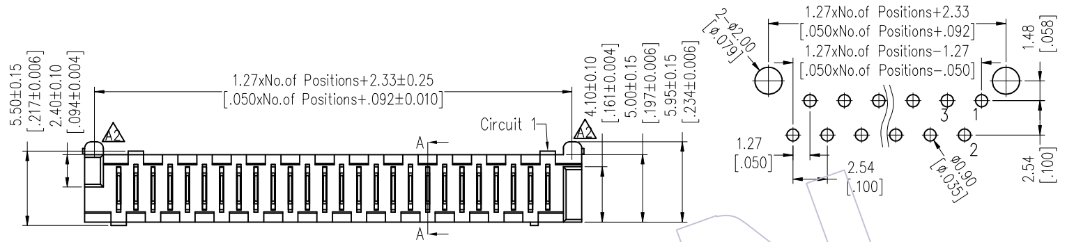
Recommended P.C.B Layout(Top Side) (PCB BOARD TOLERANCE ±0.05)
