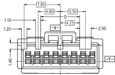
8PIN, Y-KEY
