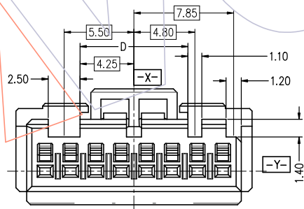
8PIN, X-KEY
