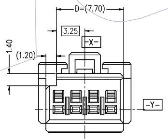
4PIN, Y-KEY
