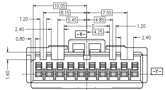
10PIN, Y-KEY
