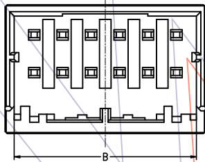
12P Y-KEY
