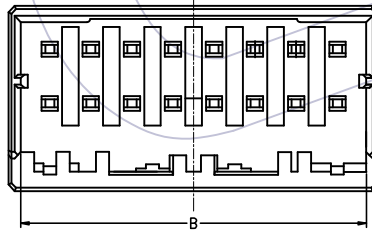
16P Y-KEY
