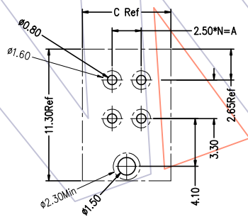
Recommended P.C.B Layout(Top Side) (PCB BOARD THICKNESS 1.0~1.6±0.05)
