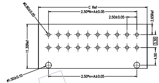
Recommended P.C.B Layout(Top Side) (PCB BOARD THICKNESS 1.0~1.6±0.05)
