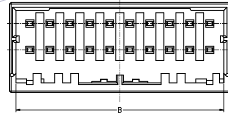
20P Y-KEY
